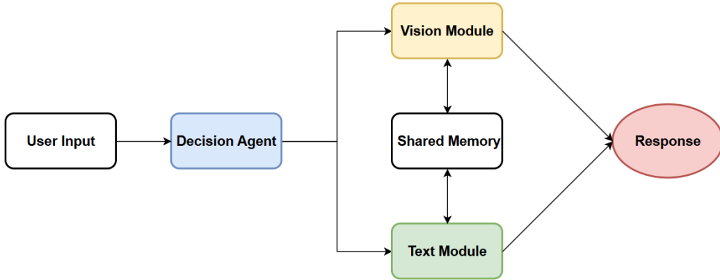
Figure 3.1: Overall architecture of the Multi-Agent Medical Assistant
