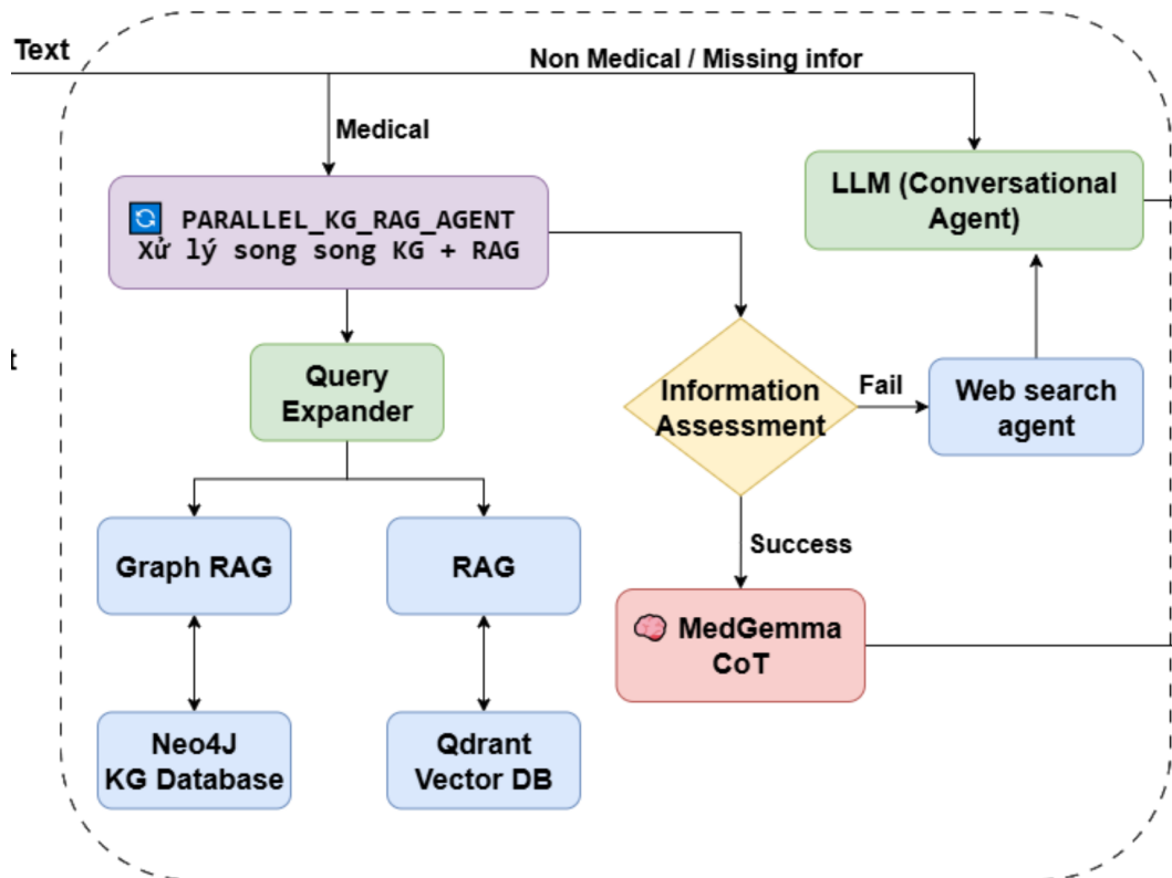
Figure 4.1: Text Module architecture for medical knowledge retrieval
