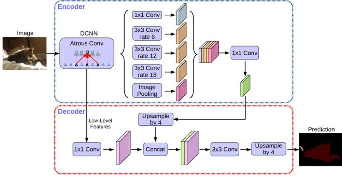
Figure 5.2: DeepLabV3+ encoder-decoder architecture with Atrous Spatial Pyramid Pooling
