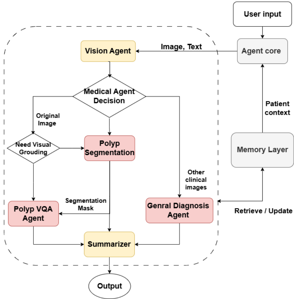
Figure 5.1: Vision Module workflow with routing, optional grounding, summarization, and memory context
