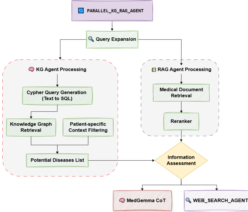
Figure 4.4: Parallel KG-RAG processing in the Text Module
