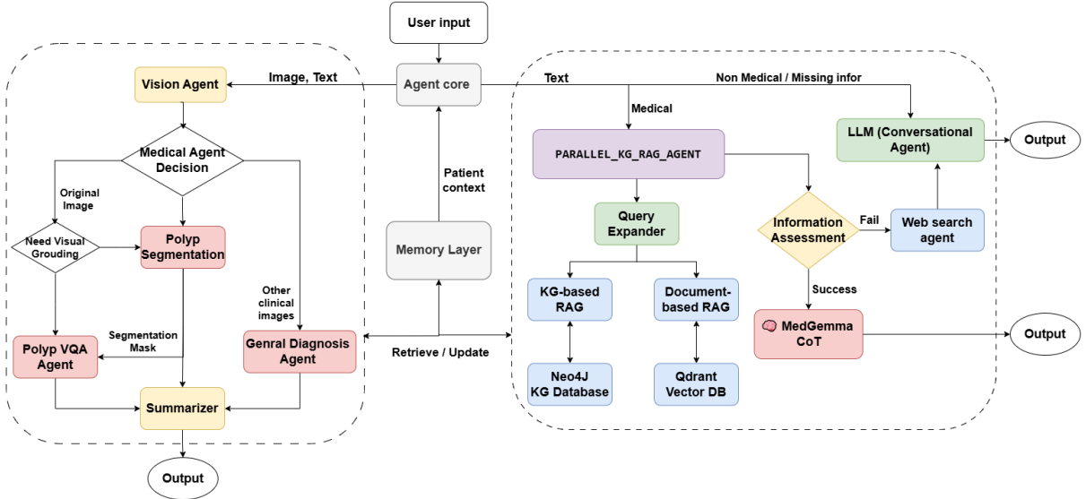
Figure 3.2: Detailed agent workflow with text, vision, memory, and fallback coordination
